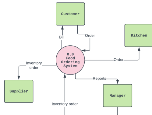
CONTEXT LEVEL FOOD ORDERING SYSTEM DATA FLOW DIAGRAM
