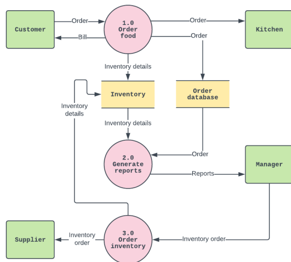
LEVEL 1 FOOD ORDERING SYSTEM DATA FLOW DIAGRAM
